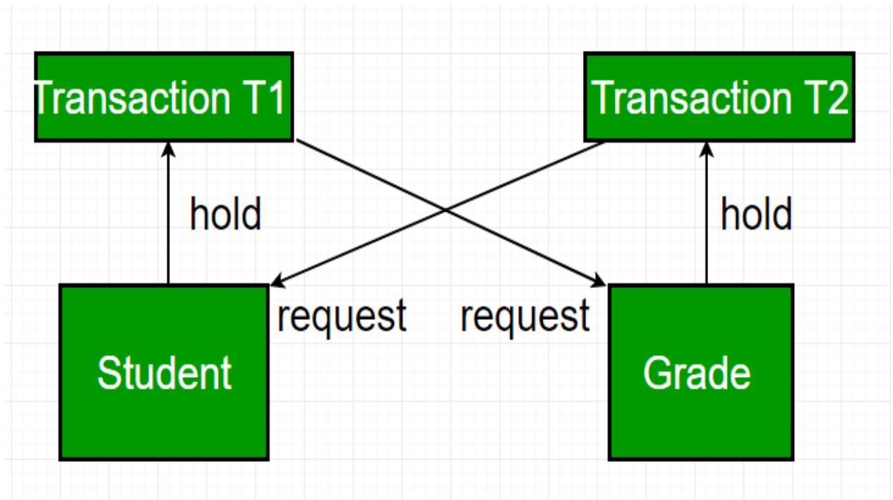
Figure 11.2: Deadlock in DBMS
