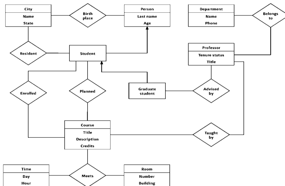
Figure 6.7: ER Diagram of University Database System
